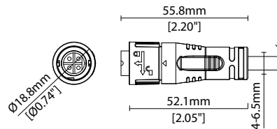
4 Pin LEDmix Male Connector IP67 (Premoulded)
