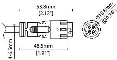
4 Pin LEDmix Female Connector IP67 (Premoulded)
